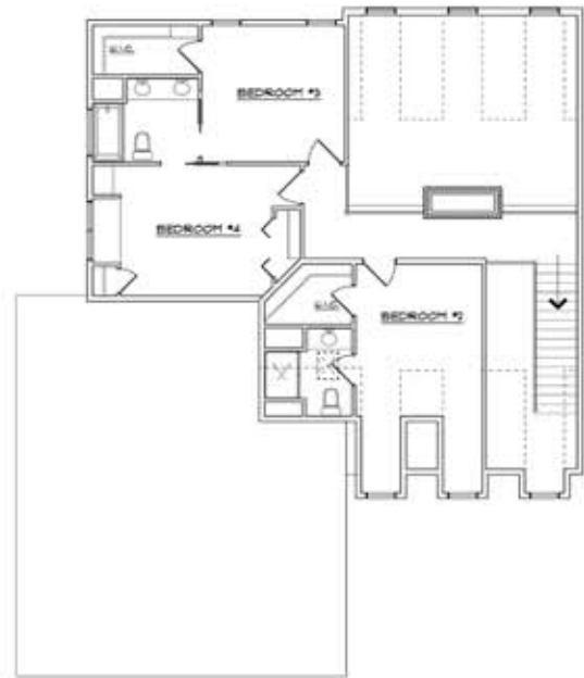
2nd Floor
